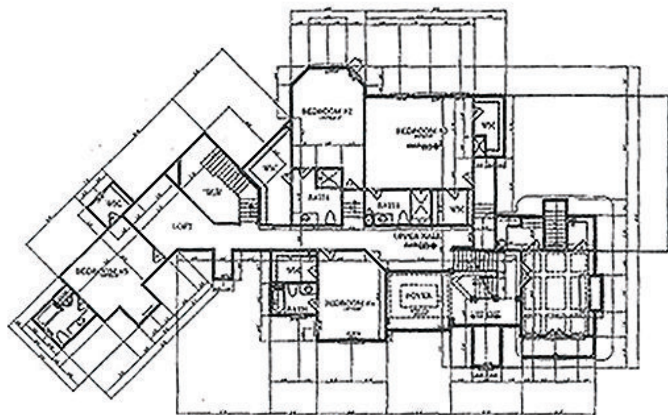
SECOND FLOOR PLAN 1/11/07 10/11/07
